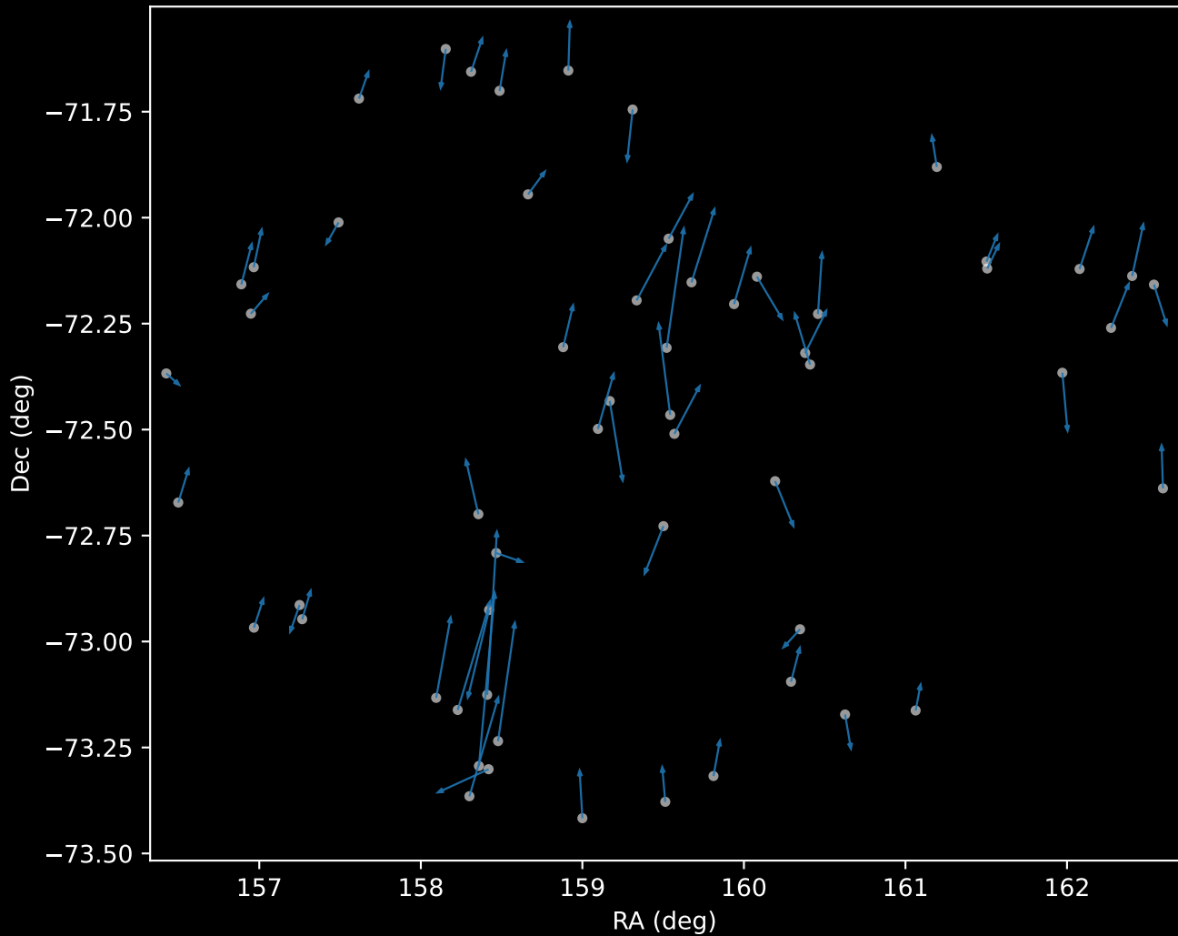
GALAH DR4 Cluster 0 Proper Motion Vectors (n=58)
