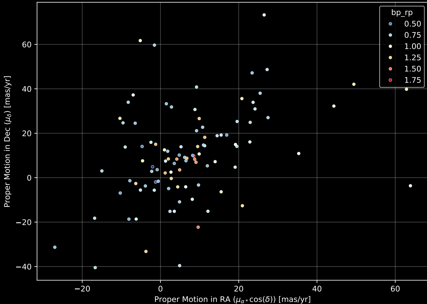
GALAH DR4 Field: [7243] Proper Motion Diagram (n= 98)
