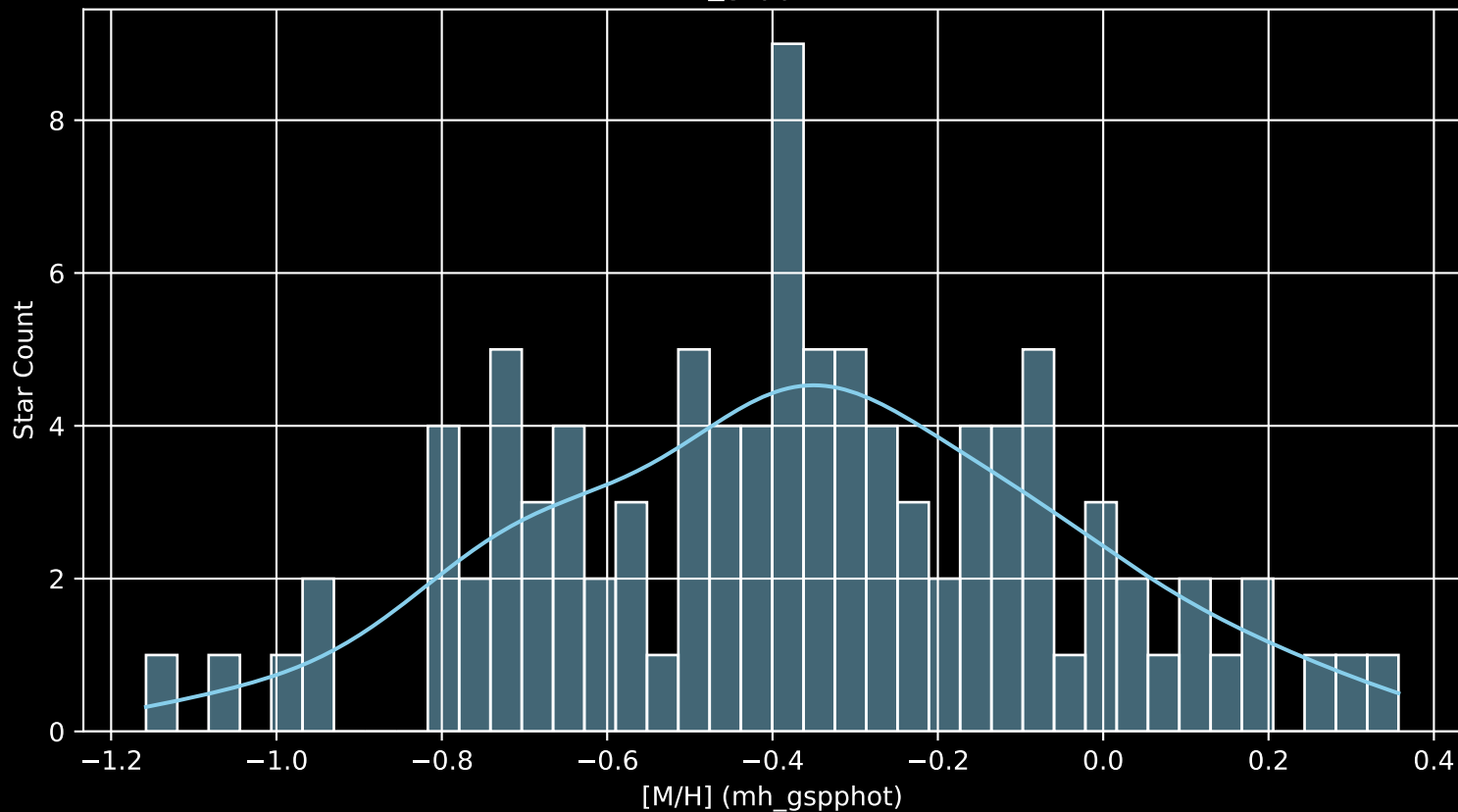
GALAH DR4 Field: [7243] [M/H] (mh_gspphot) (n= 98)
