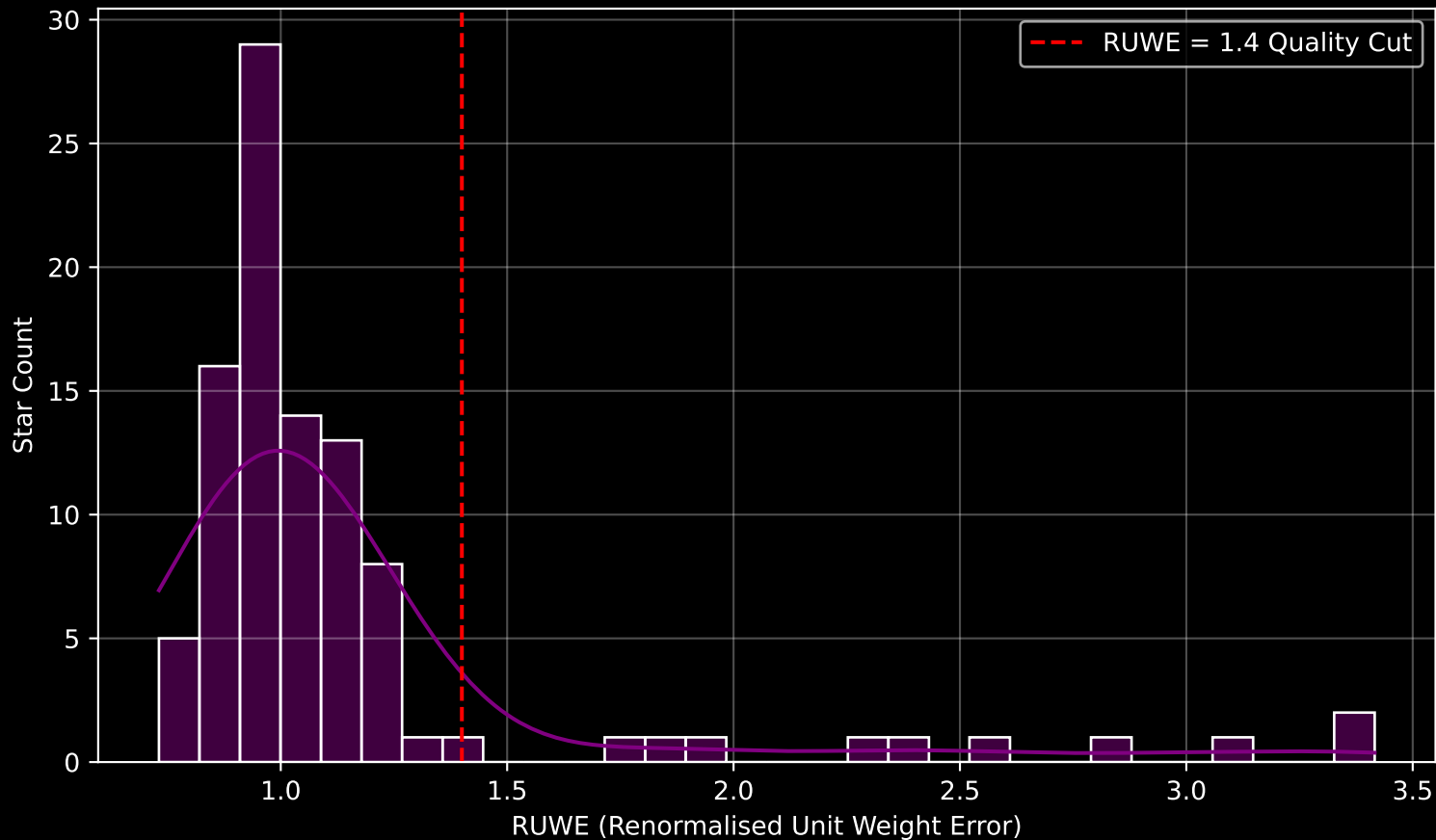
GALAH DR4 Field [7243] RUWE Distribution (n= 97)
