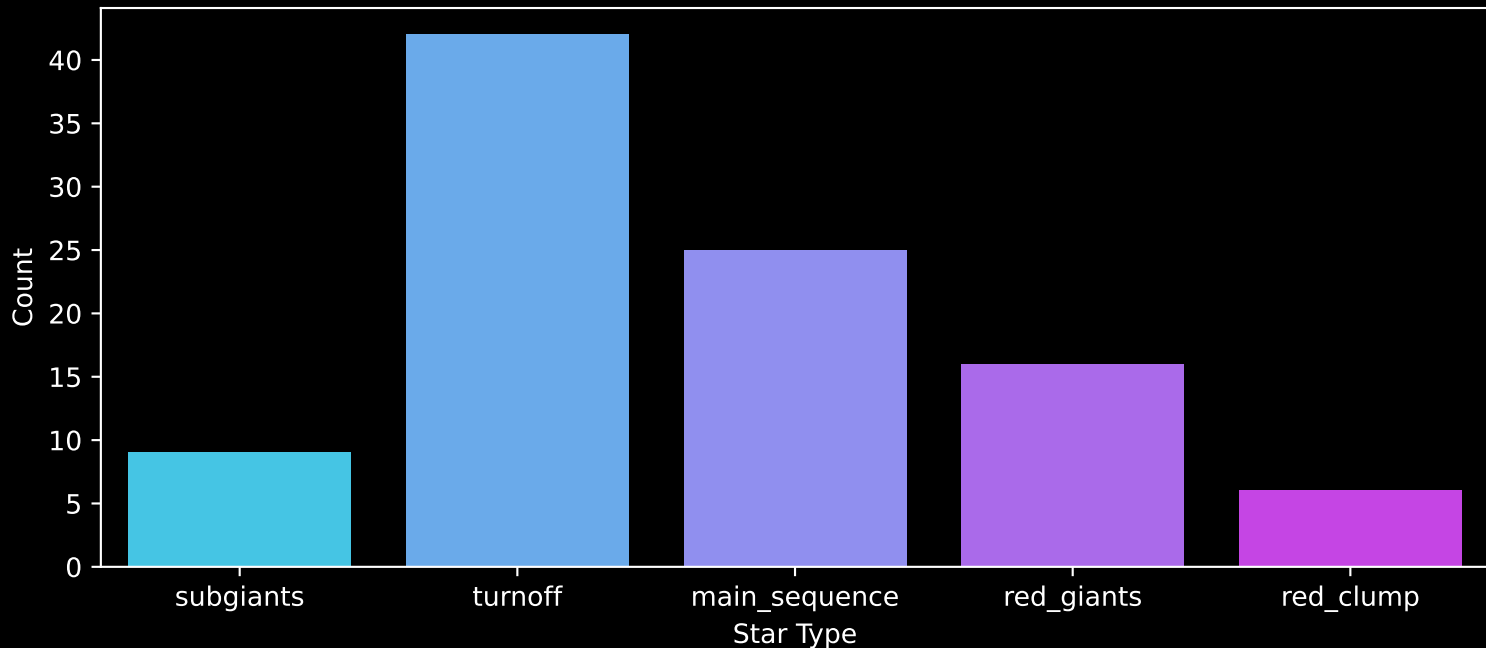
GALAH DR4 Field: [7243] Count plot of Star Type
