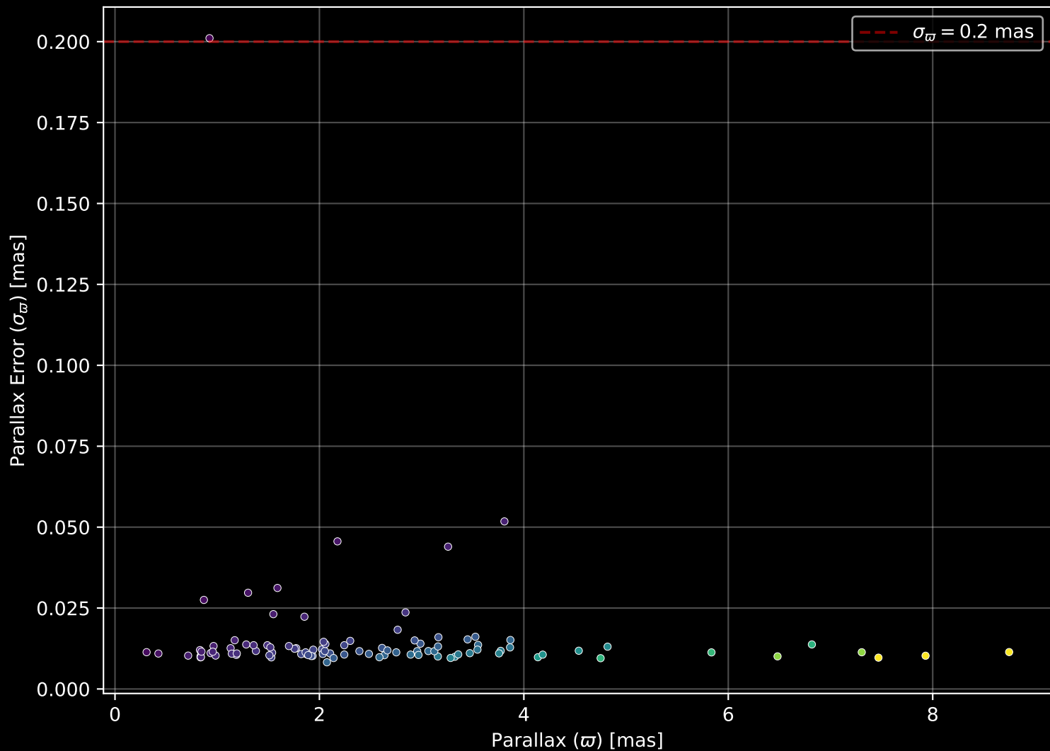
GALAH DR4 Field: [7243] Parallax Quality (n= 98)
